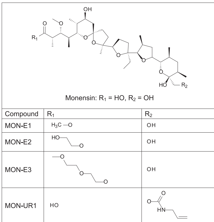
Fig. 2 Structure of monensin and its derivatives studied in this work
